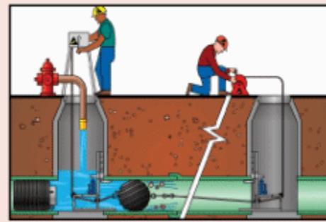
3) Introduce water into manhole and slowly release Jet-Ball® down the line.
